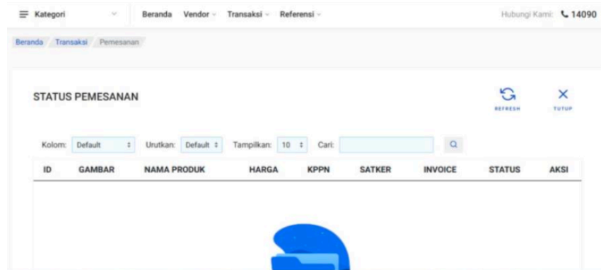
Figure 2. Order Status
